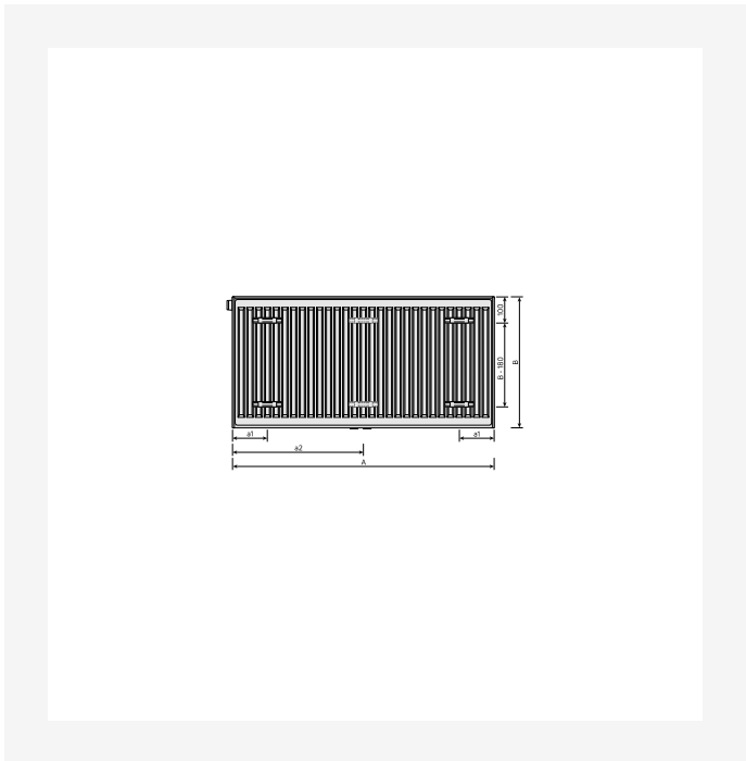
Flex, type 21, 22, 33, baksidesvy
