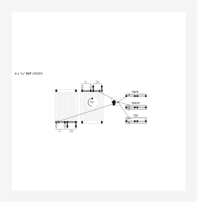
Vertical Connection Options
