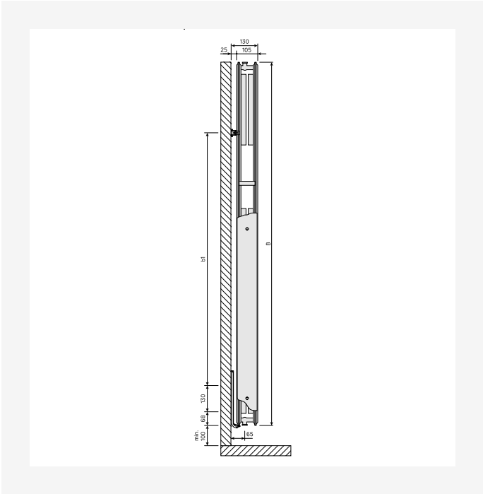
New_Vertical side view
