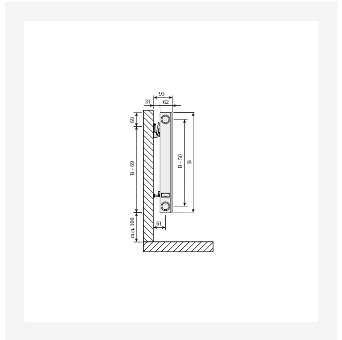
Dimensional drawing
