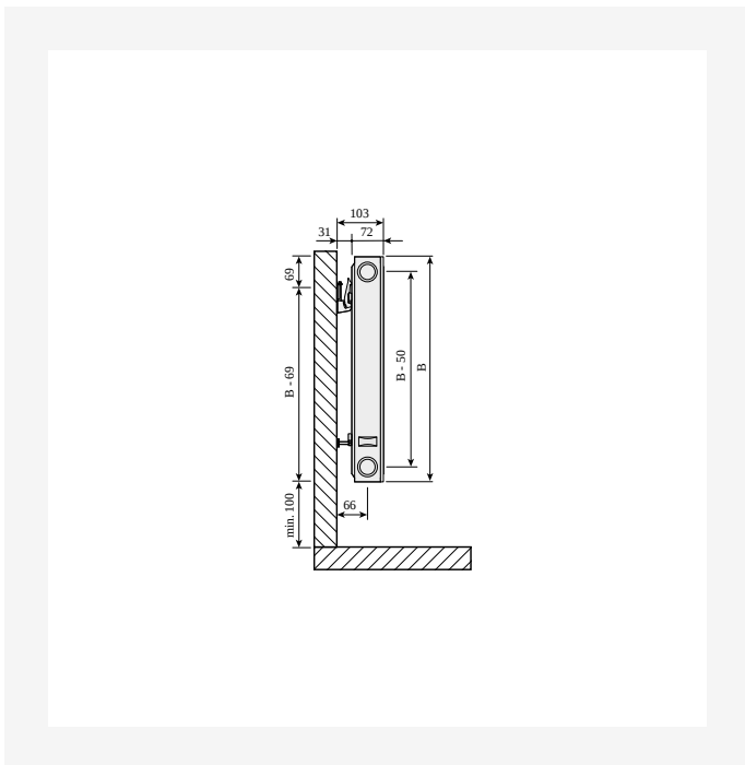
Dimensional drawing
