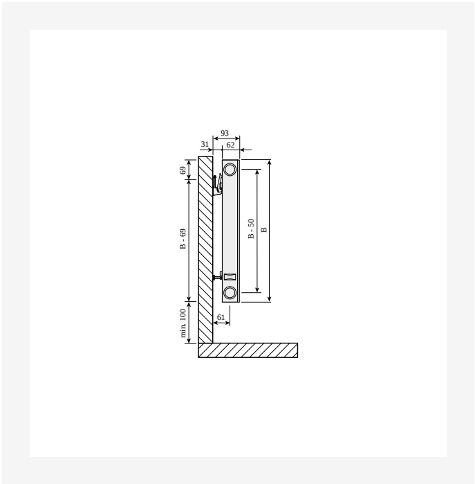
Dimensional drawing
