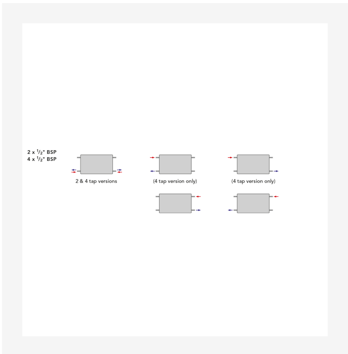
Premier HE Connection Options
