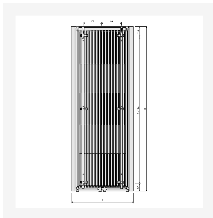
Plan Coté - New_Paros V_RV_T11_MCWV_0124
