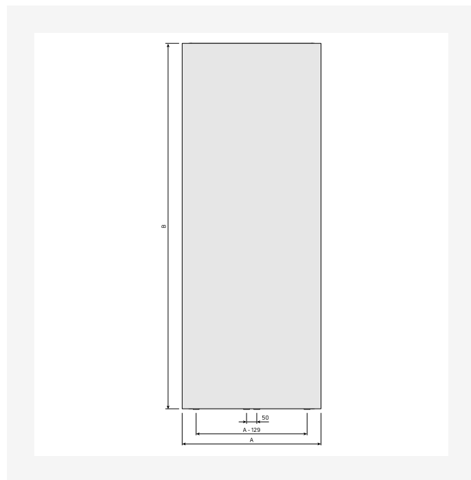
Plan Coté - New_Paros V_FV_T11_0124
