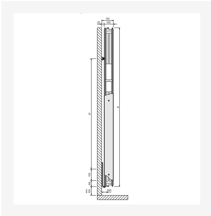
Dimensietekening - New_Vertical_SV_T22_0124
