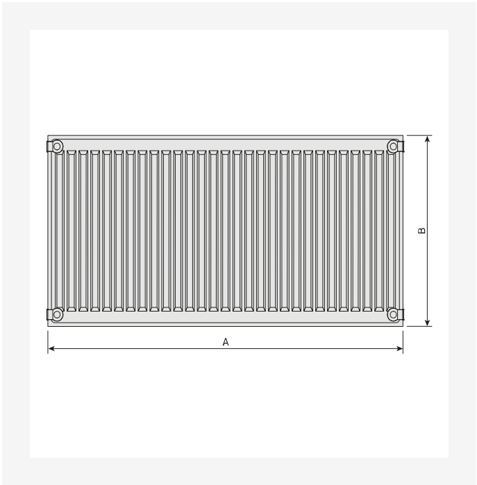
Dimensional Drawing - PR-Hygiene-RV-T10-0924
