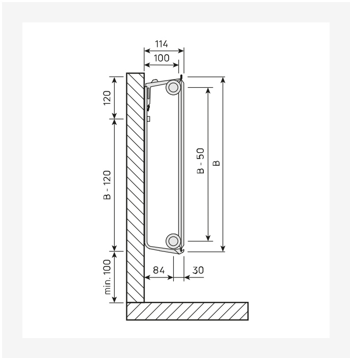
Dimensional Drawing - PR-Hygiene-T10-SV-0220
