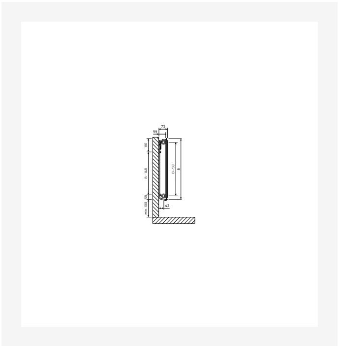
Dimensional Drawing - PR-Hygiene-T10-SV-MCK66-0121
