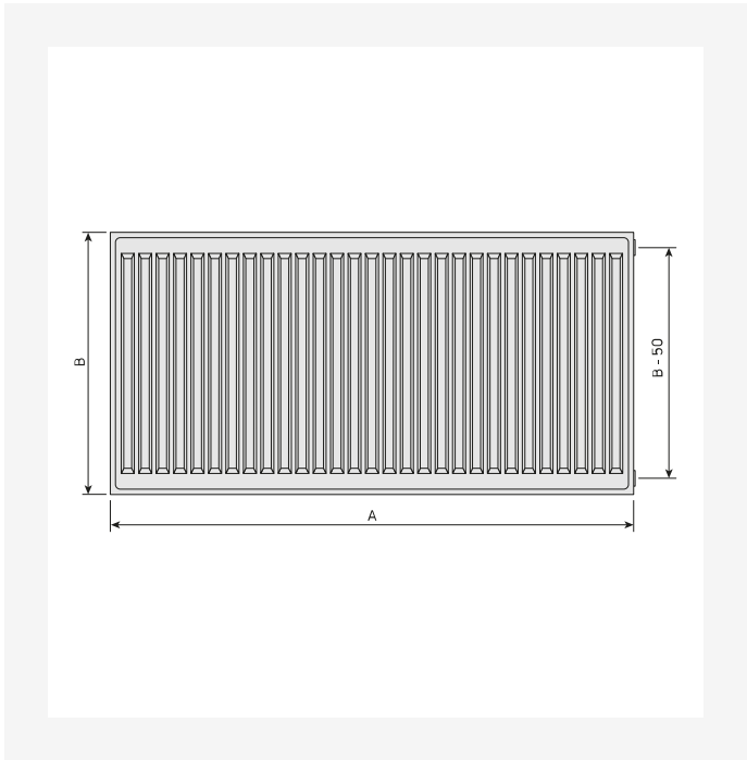
Dimensional Drawing - PR-Hygiene-FV-0220
