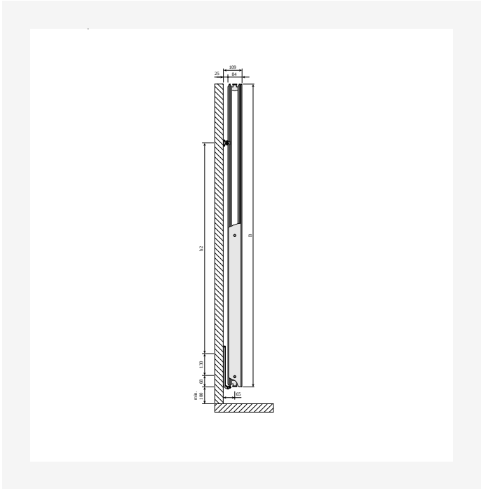
Dimensional Drawing - PR-KOV-FAV-T20-SV-0120
