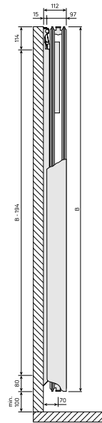
Dimensional Drawing - New_Tinos V-Paros V_SV_T21_0124
