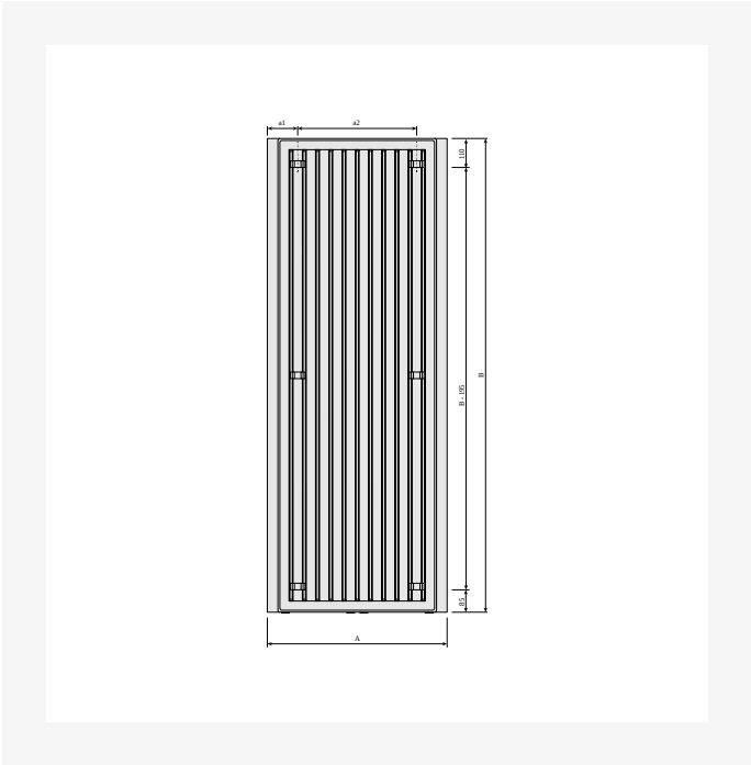
Dimensional Drawing - PR-PAV-BV-0320
