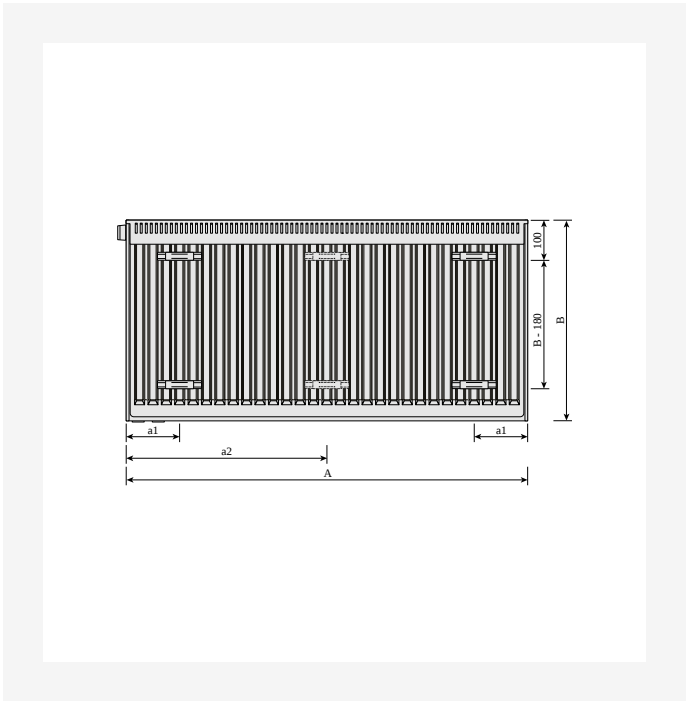
Dimensional Drawing - PR-Plan-Ventil-Compact-T11-BV-0220
