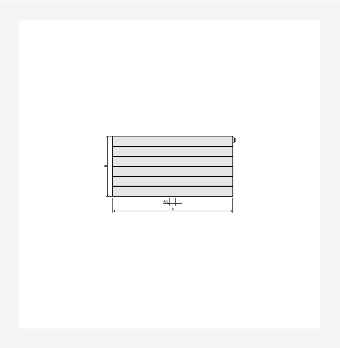
Dimensional Drawing - Ramo_Flex-FV-1221
