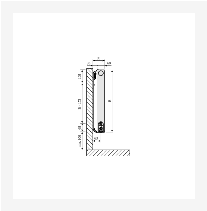
Dimensional Drawing - PR-Termopanel-TP11-SV-Monclac42-0320
