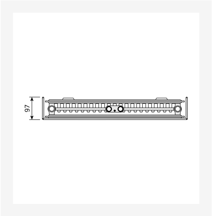
Dimensional Drawing - New_Tinos V_TV_T21_0124
