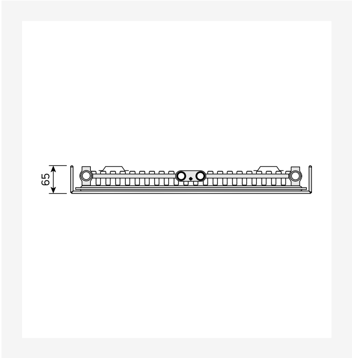
Dimensional Drawing - New_Tinos V_TV_T11_0124
