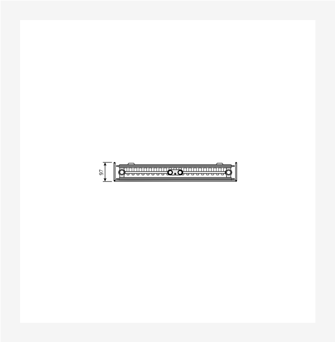
Dimensional Drawing - PR-TIV-T21-TV-0320
