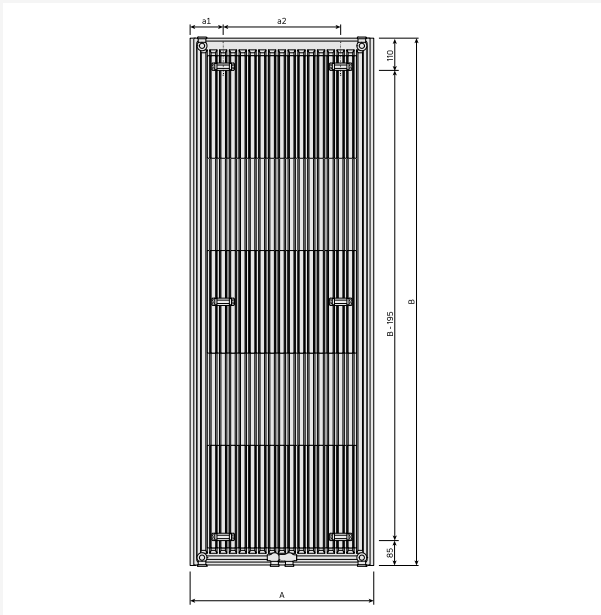
Dimensional Drawing - New_Tinos V_RV_T11_0124
