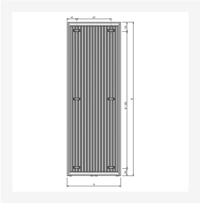
Dimensional Drawing - New_Tinos V_RV_T21_0124
