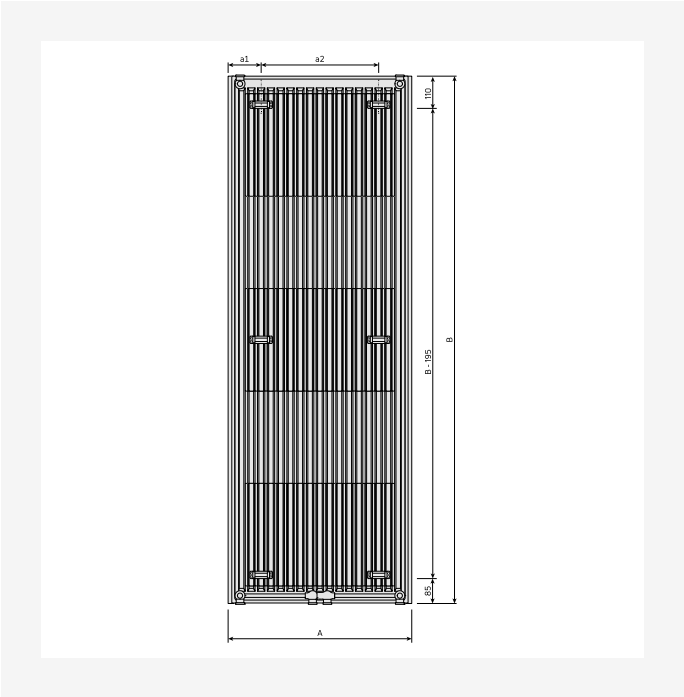
Dimensional Drawing - New_Tinos V_RV_T11_0124
