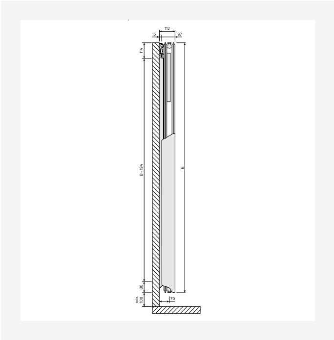
Dimensional Drawing - New_Tinos V-Paros V_SV_T21_0124
