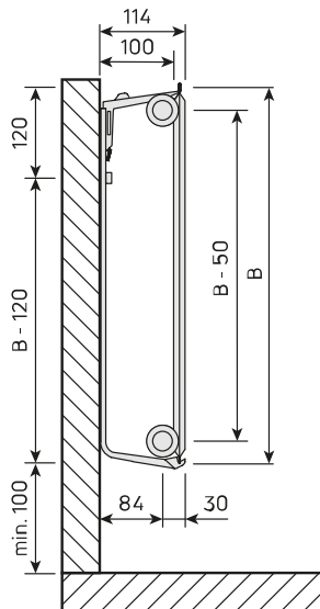
Dimensional Drawing - PR-Hygiene-T10-SV-0220
