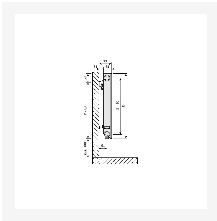
Dimensional Drawing - PR-Plan-Ventil-Compact-Ramo-Ventil-Compact-T11-SV-0220
