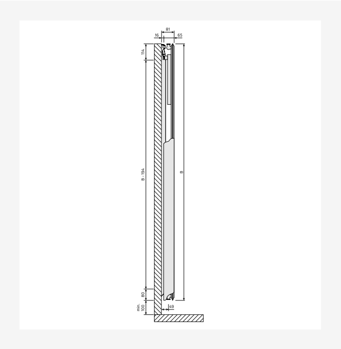
Dimensional Drawing - New_Tinos V-Paros V_SV_T11_0124
