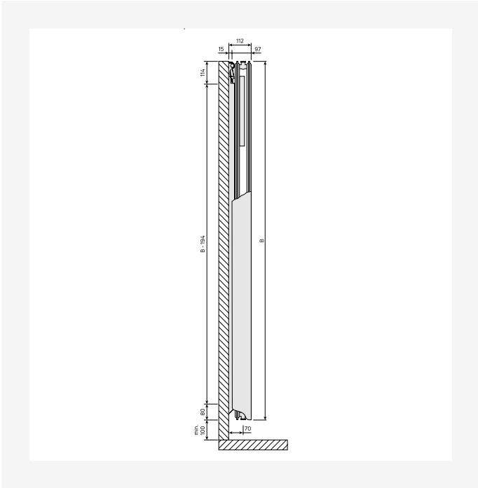
Dimensional Drawing - New_Tinos V-Paros V_SV_T21_0124
