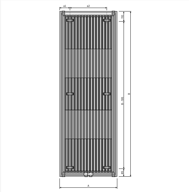
Dimensional Drawing - New_Tinos V_RV_T11_0124
