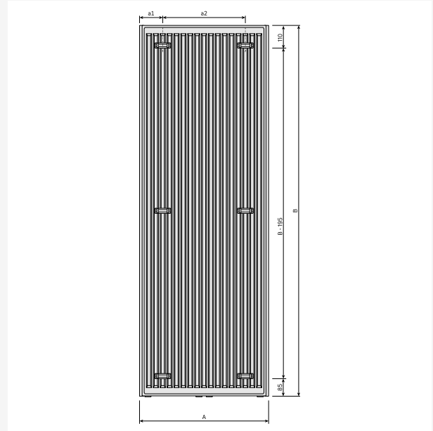
Dimensional Drawing - New_Tinos V_RV_T21_0124
