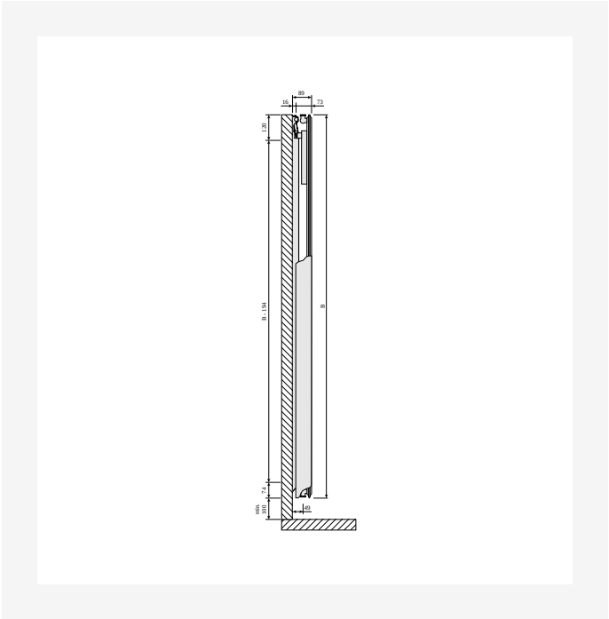
Dimensional Drawing - PR-TIV-T11-SV-0320
