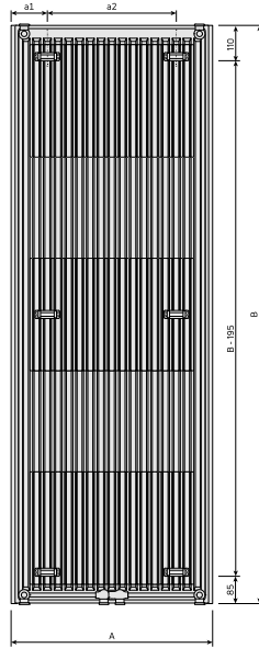
Dimensional Drawing - New_Tinos V_RV_T11_0124
