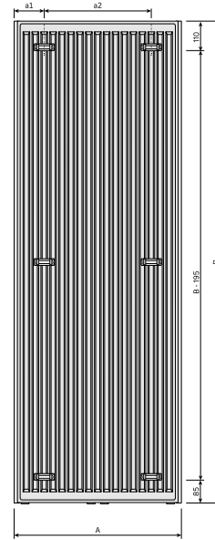
Dimensional Drawing - New_Tinos V_RV_T21_0124
