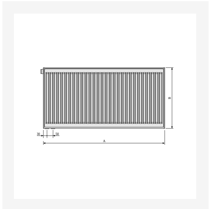
Dimensional Drawing - Ventil Compact, tyypit 20, 21s, 22, 30, 33, takaa katsottuna
