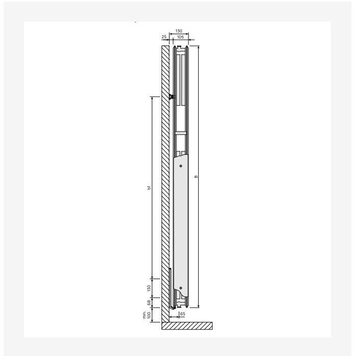
Dimensietekening - New_Vertical_SV_T22_0124
