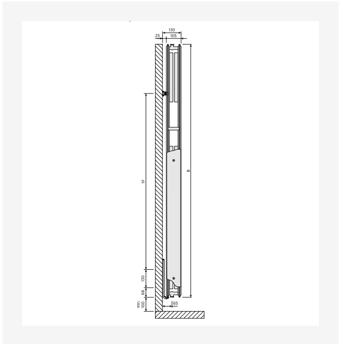
Dimensietekening - New_Vertical_SV_T22_0124
