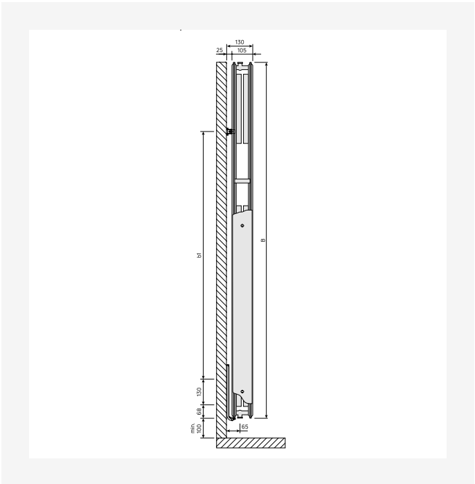
Dimensietekening - New_Vertical_SV_T22_0124
