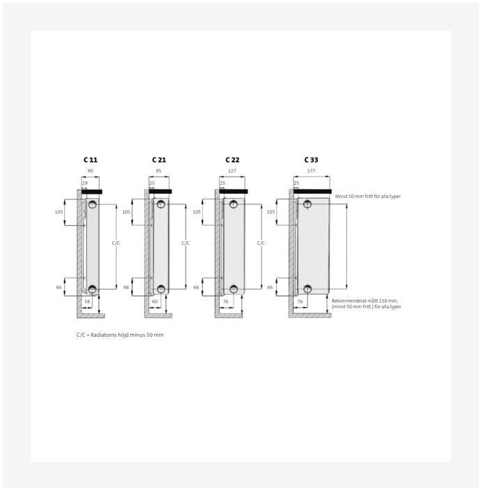
Dimensional Drawing - 1.12 Installationsmått
