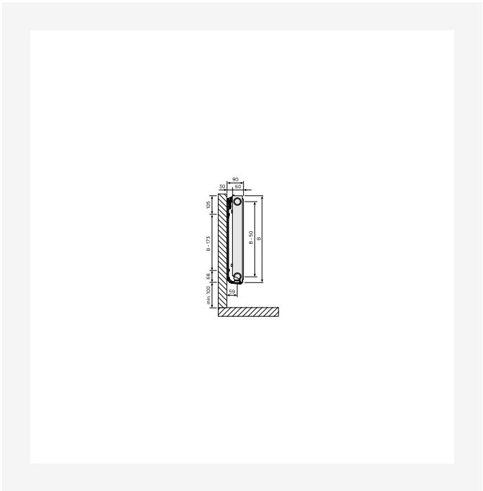
Dimensional Drawing - CVF, type 11, sidevisning monclac
