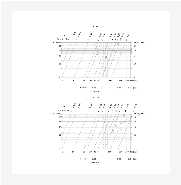
Installation Instructions - fla_valve_diagram KVS KV DT2K with sound diagram
