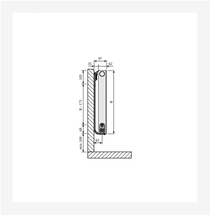
Dimensional Drawing - PR-Thermopanel-TP-Plan-TP-Ramo-T11-SV-Monclac42-0320
