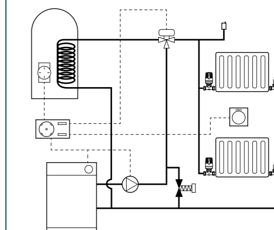
3 port valve system diagram
