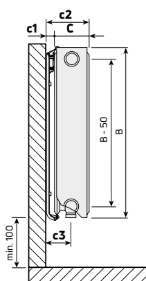
B ≥ 300 mm types 21s, 22, 33
