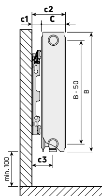
B ≥ 400 mm type 11
