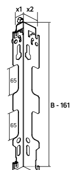
B ≥ 400 mm type 11
