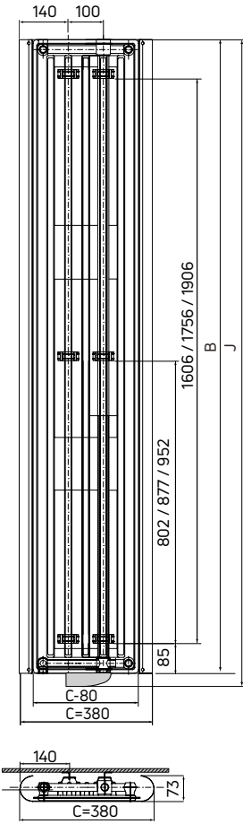
type 11 (380 mm)
