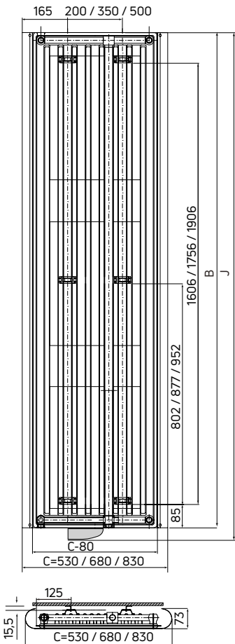
type 11 (530 / 680 / 830 mm)
