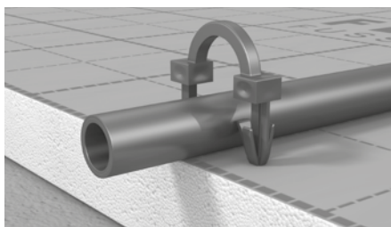
Abb. 4: Tackerclips 3D
